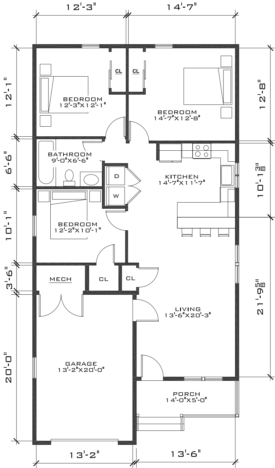
① SINGLE FAMILY HOUSE TYPE 1 - 1,418 SF 1/8" = 1'-0"
