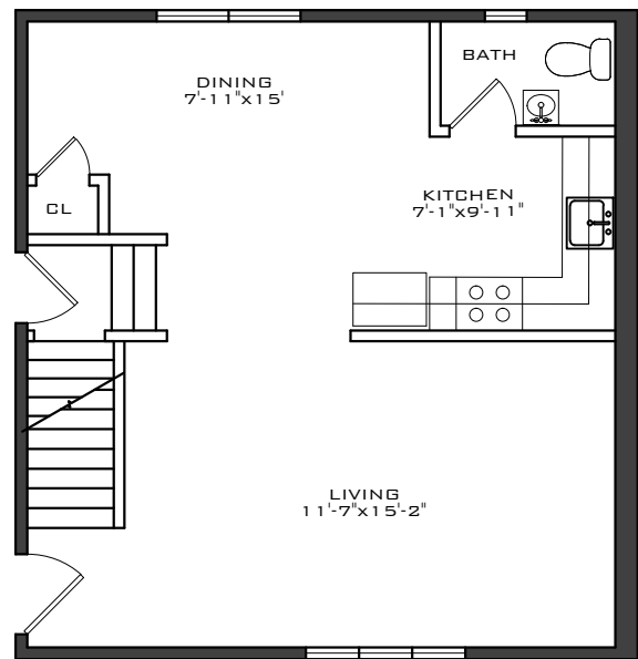
② UNIT 431 - 1ST FLOOR 1/8" = 1'-0"
