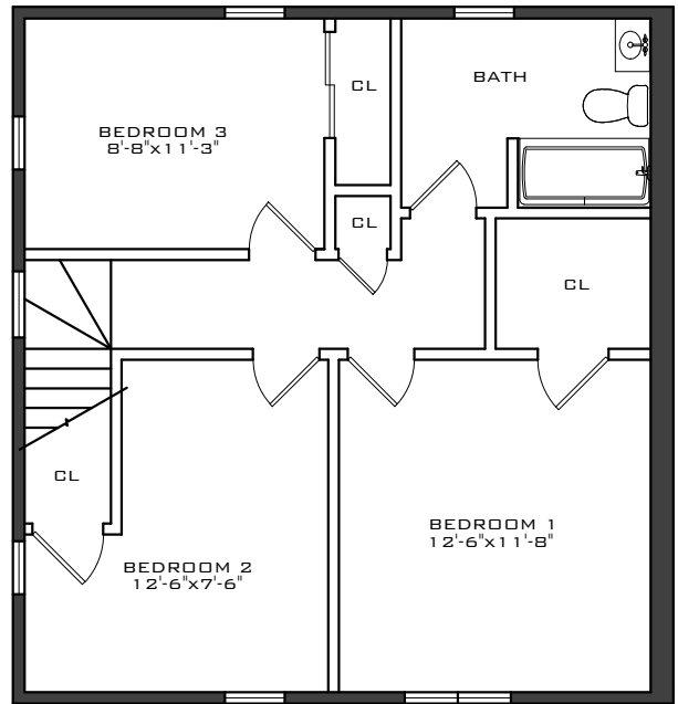
③ UNIT 470- 2ND FLOOR 1/8" = 1'-0"
