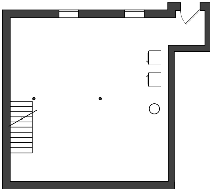
① UNIT 431 - BASEMENT 1/8" = 1'-0"
