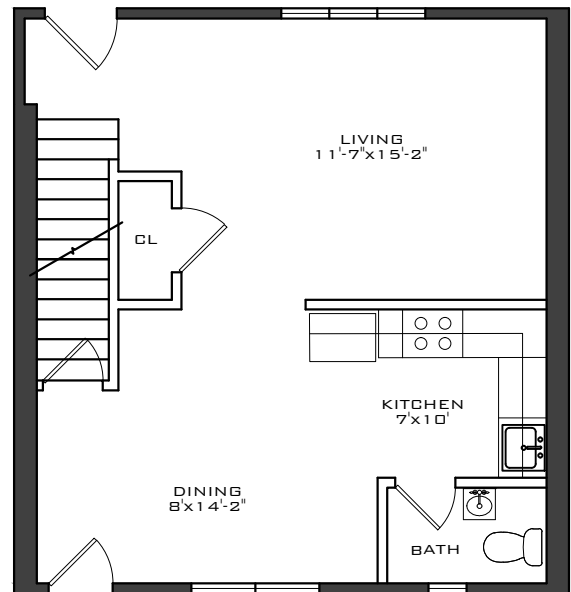
② UNIT 426 - 1ST FLOOR 1/8" = 1'-0"
