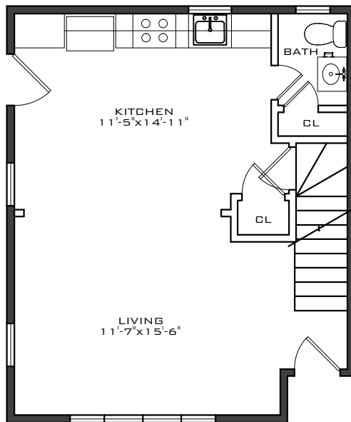
② UNIT 371-A - 1ST FLOOR 1/8" = 1'-0"
