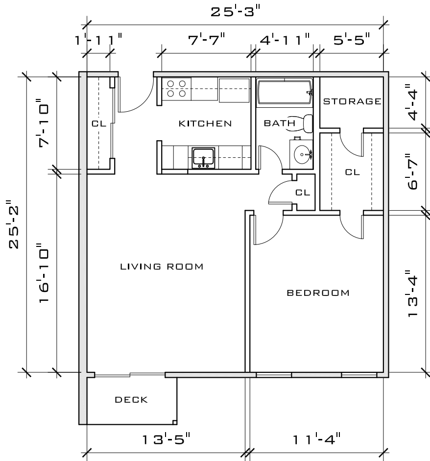
① UNIT TYPE B 1/8" = 1'-0"
