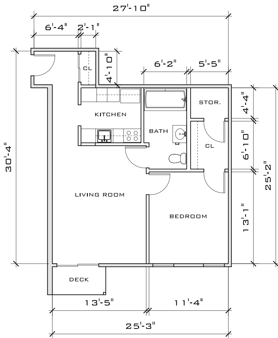
① UNIT TYPE F 1/8" = 1'-0"
