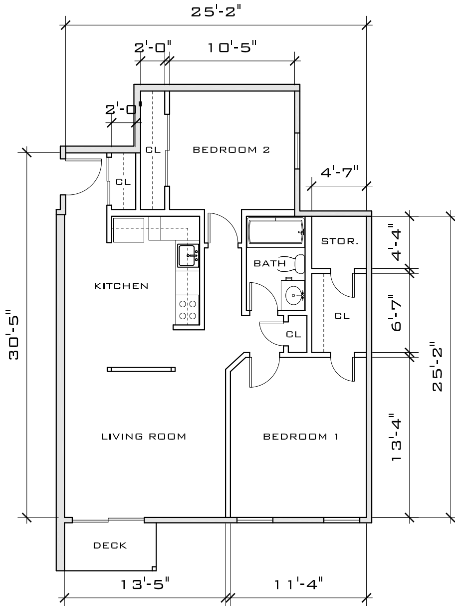
① UNIT TYPE C 1/8" = 1'-0"
