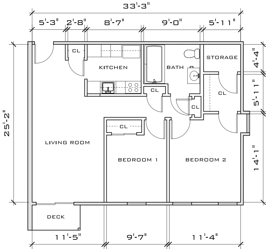
① UNIT TYPE E 1/8" = 1'-0"
