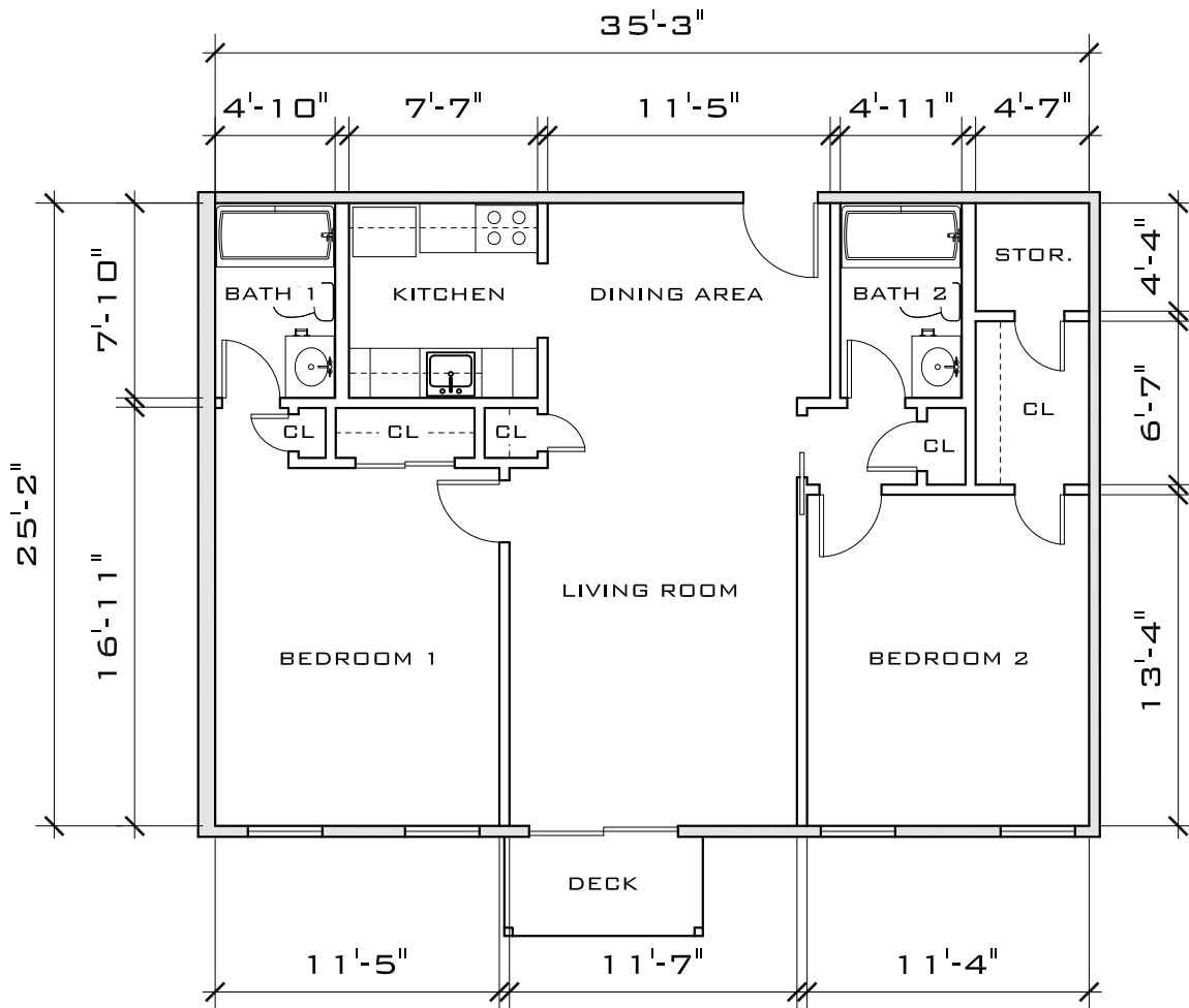
① UNIT TYPE D 1/8" = 1'-0"
