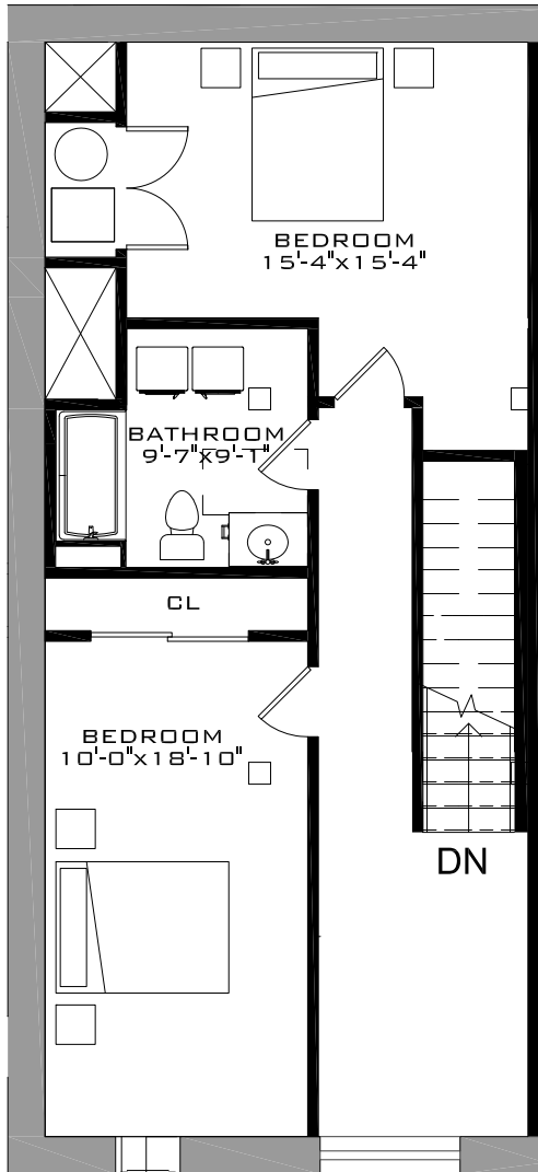
UNIT TYPE D-1.1 - UPPER LEVEL
