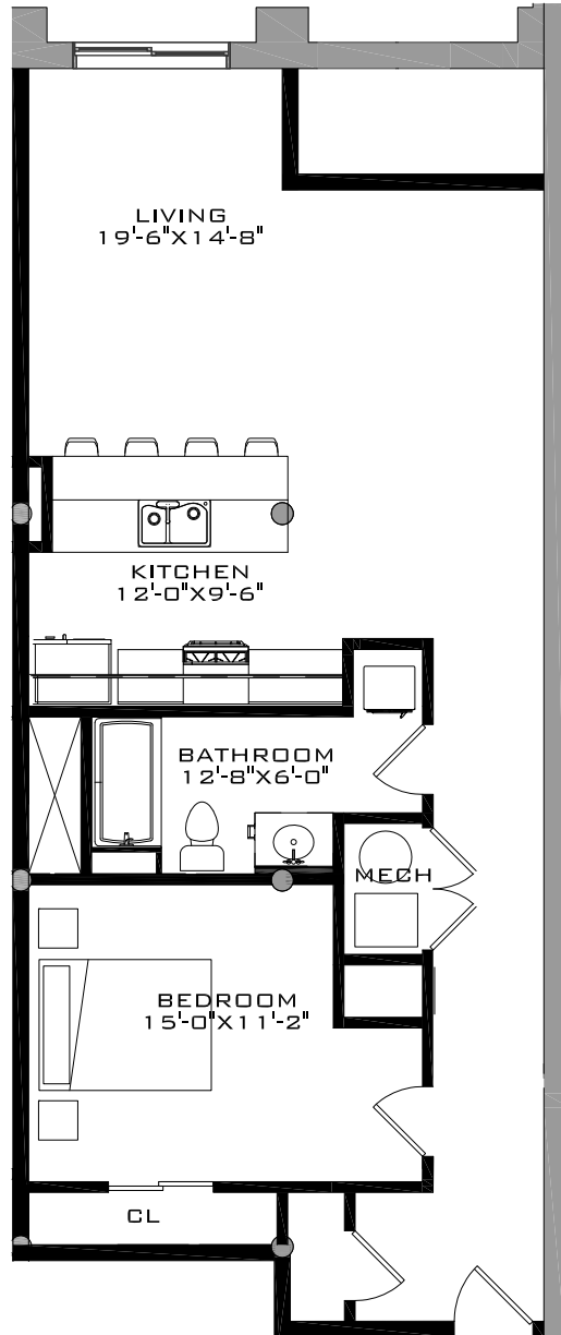
① UNIT LL01 TYPE A-2.1 - 867 SF 1/8" = 1'-0"
