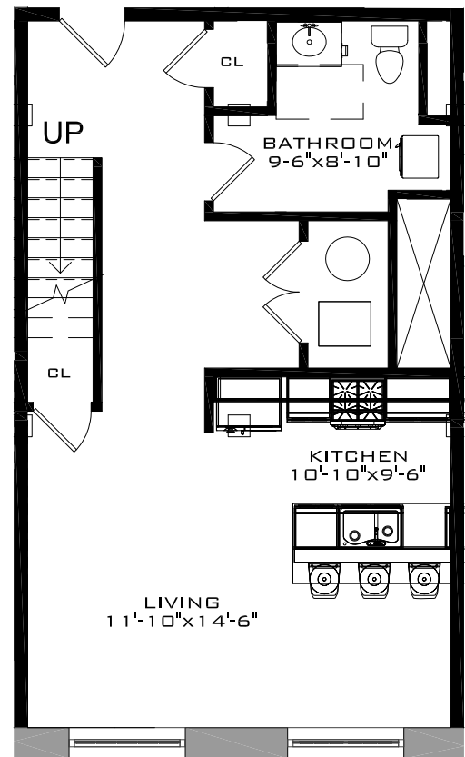
UNIT TYPE D-6.1 - LOWER LEVEL
