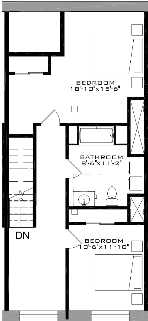
UNIT TYPE D-1.2 - UPPER LEVEL
