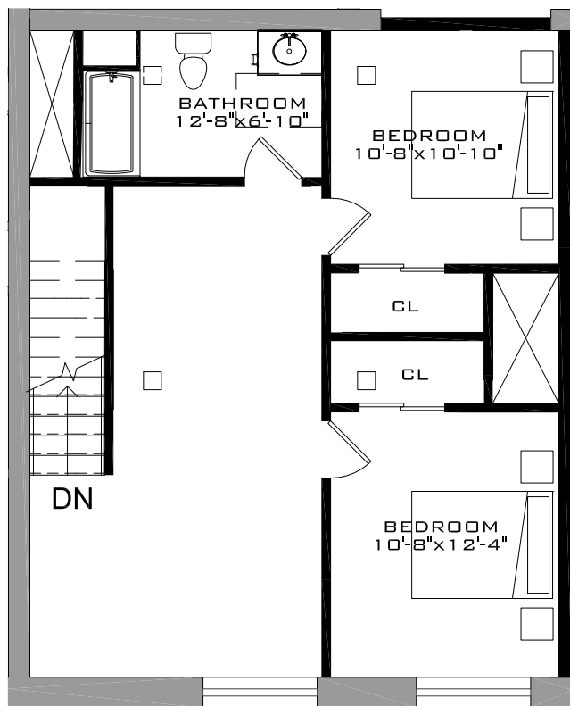
UNIT TYPE D-3.1 - UPPER LEVEL
