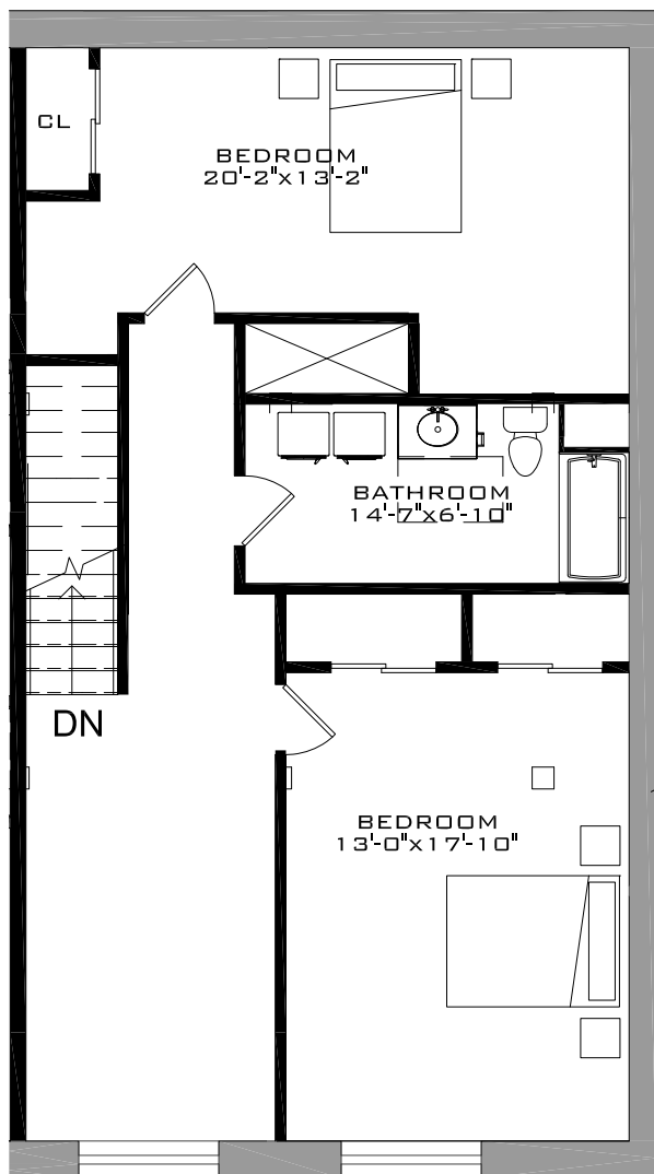
UNIT TYPE D-2.1 - UPPER LEVEL
