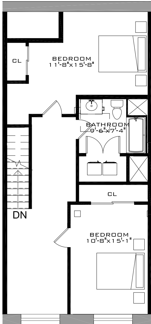
UNIT TYPE D-6.1 - UPPER LEVEL
