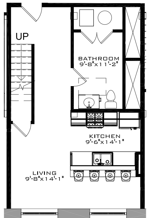
UNIT TYPE D-1.2 - LOWER LEVEL
