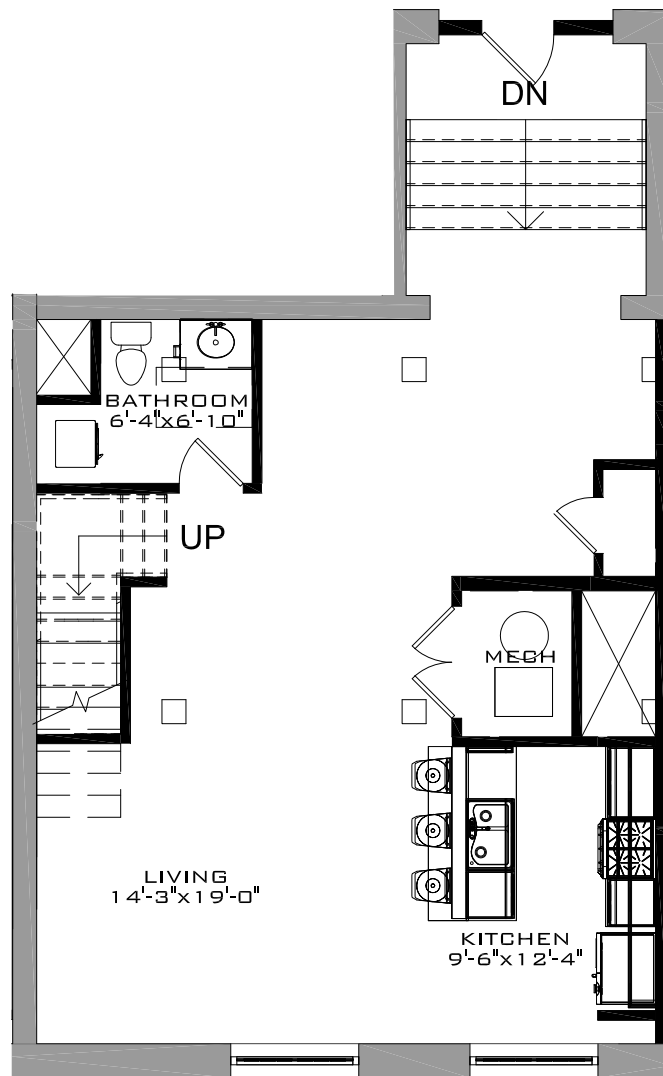
UNIT TYPE D-3.1 - LOWER LEVEL
