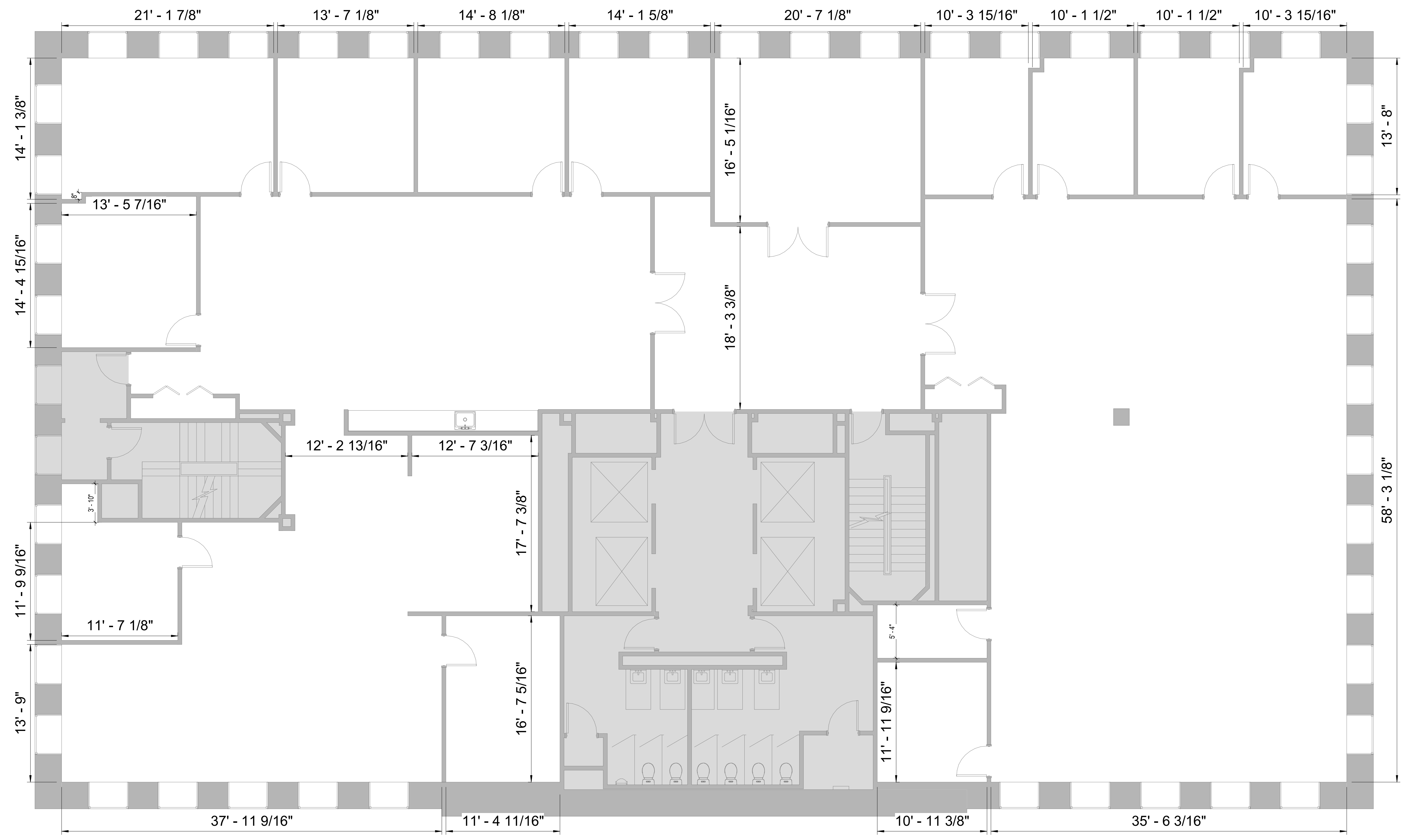
1 9th Floor - Existing Plan 3/16" = 1'-0"
