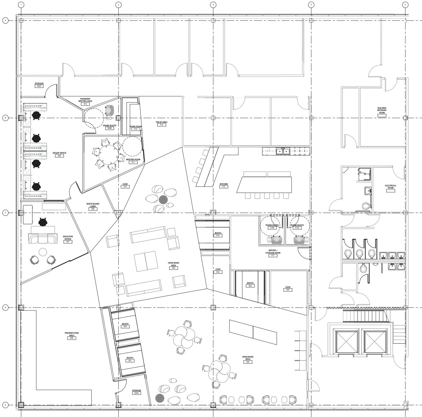
1 FIFTH FLOOR FURNITURE PLAN 1/4" = 1'-0"
