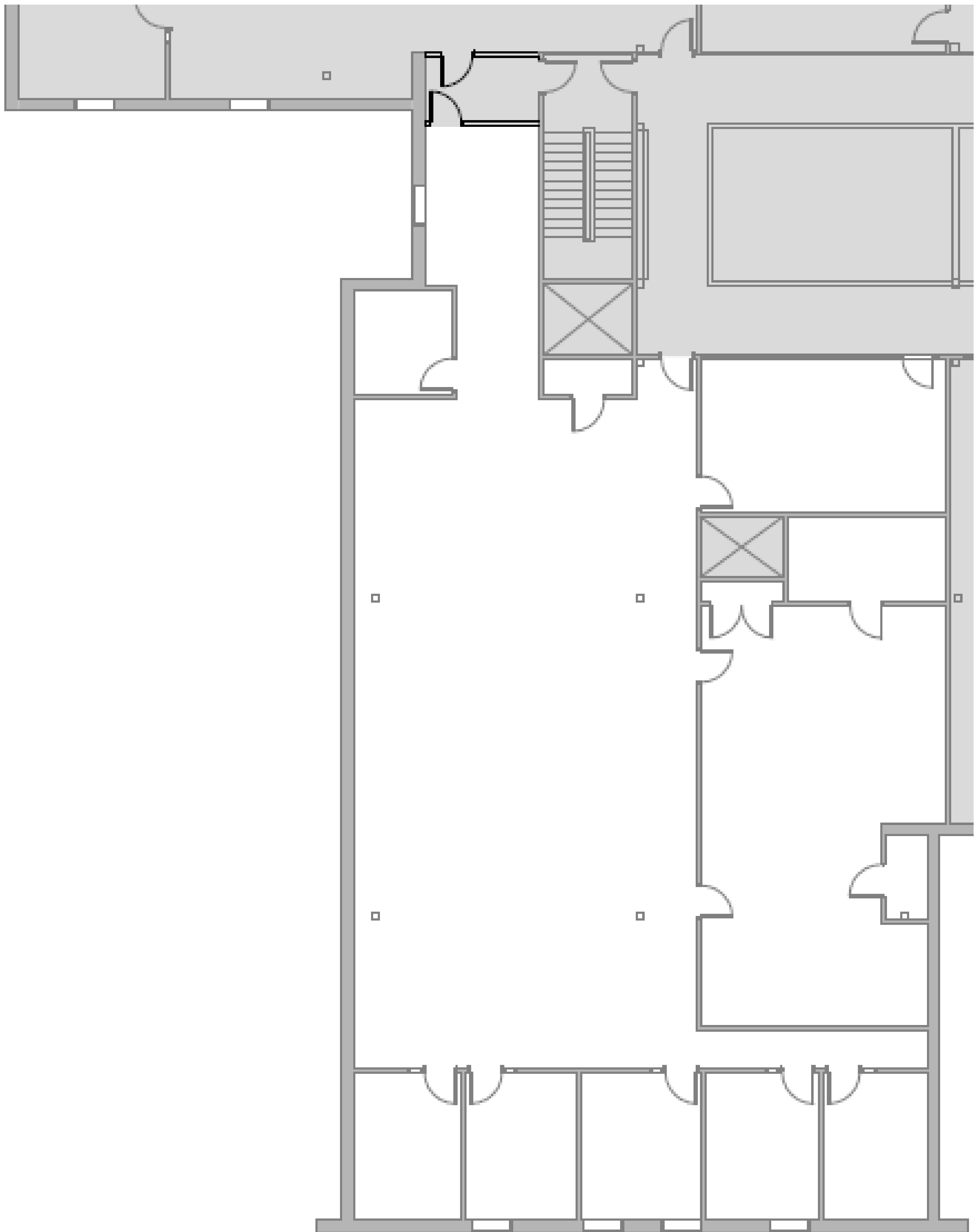
1 3RD FLOOR - FAIRCHILD EXISTING PLAN 1/8" = 1'-0"
