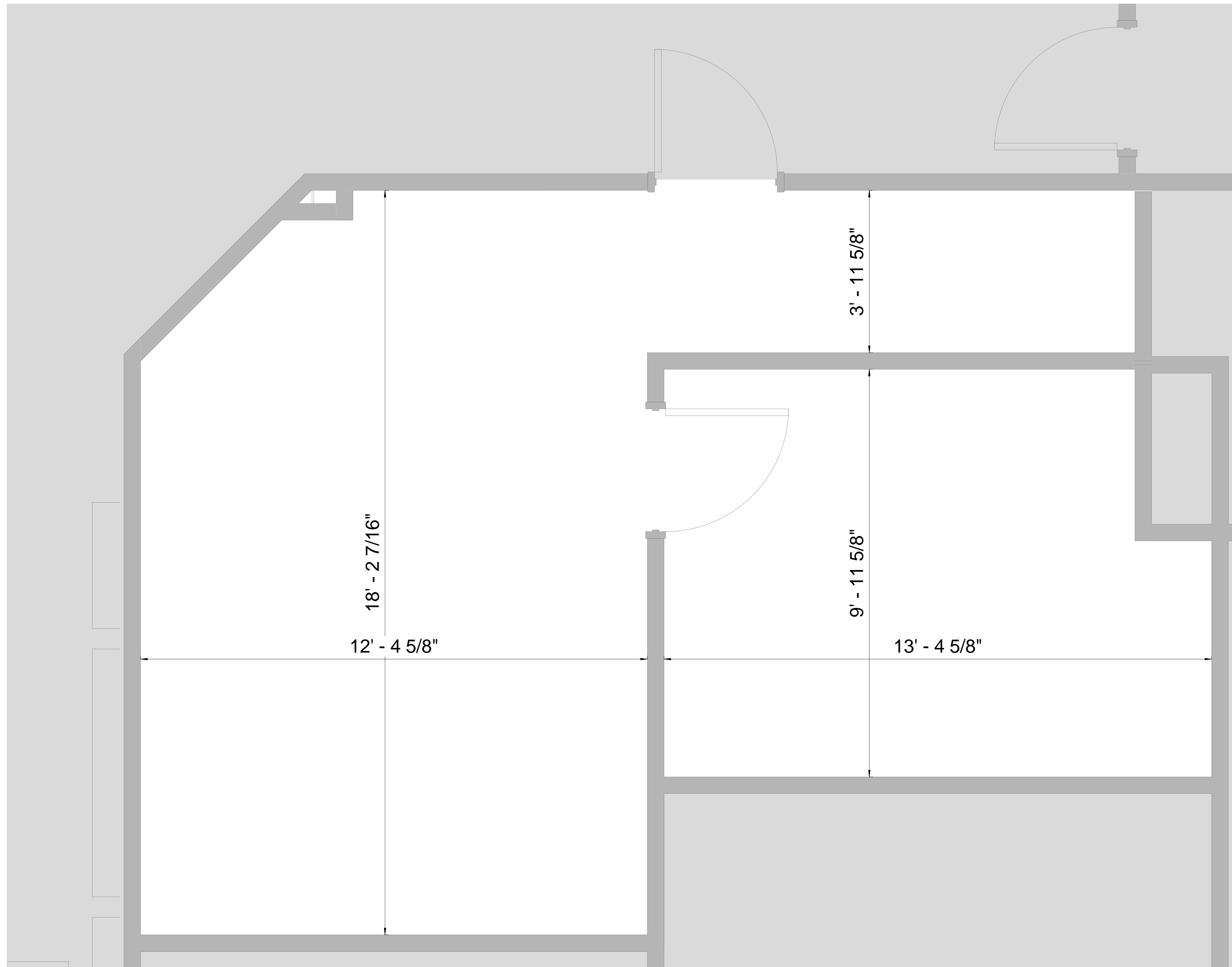
1 OLD SECURITY SPACE 3/4" = 1'-0"
