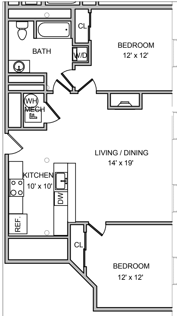
① C215 1/8" = 1'-0" SIMILAR TO UNITS C316 & C416
