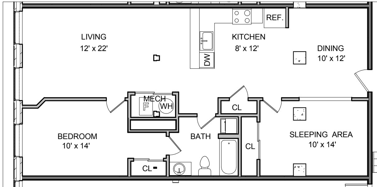
1 B001 1/8" = 1'-0" SIMILAR TO UNITS B002 & B003
