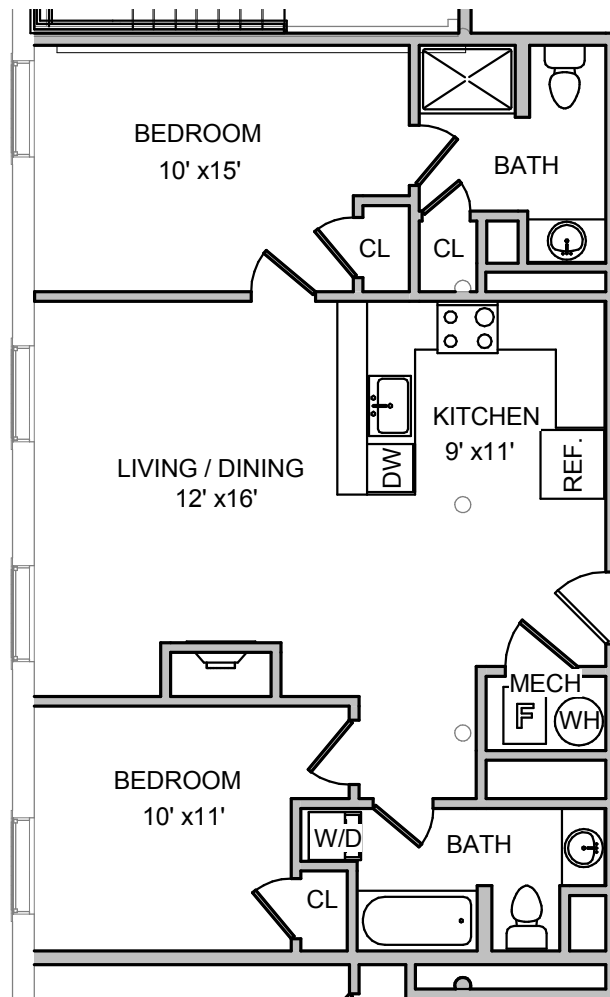
① C208 1/8" = 1'-0" SIMILAR TO UNITS C309 & C409
