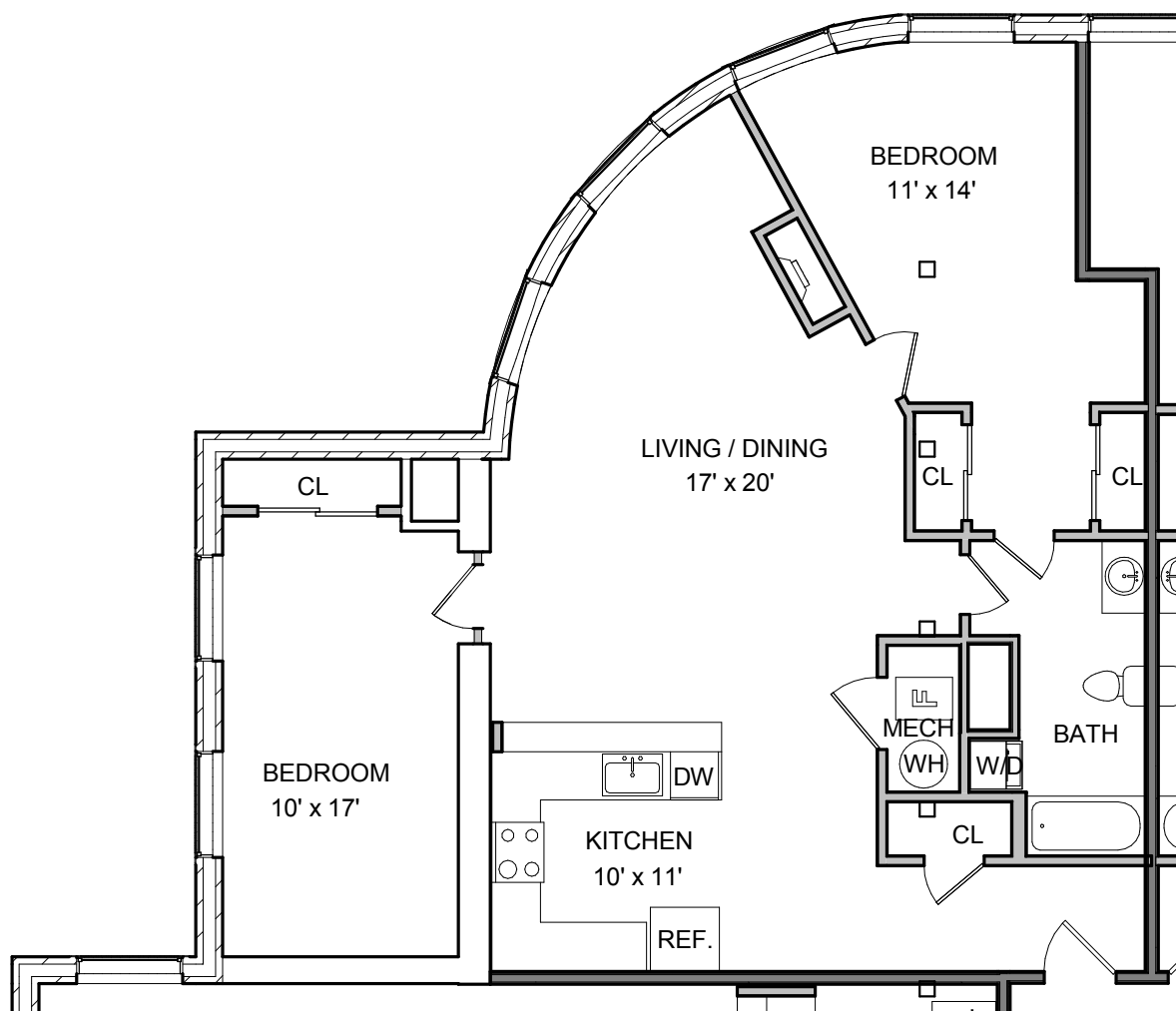
① B104 1/8" = 1'-0" SIMILAR TO UNITS B004 & B204
