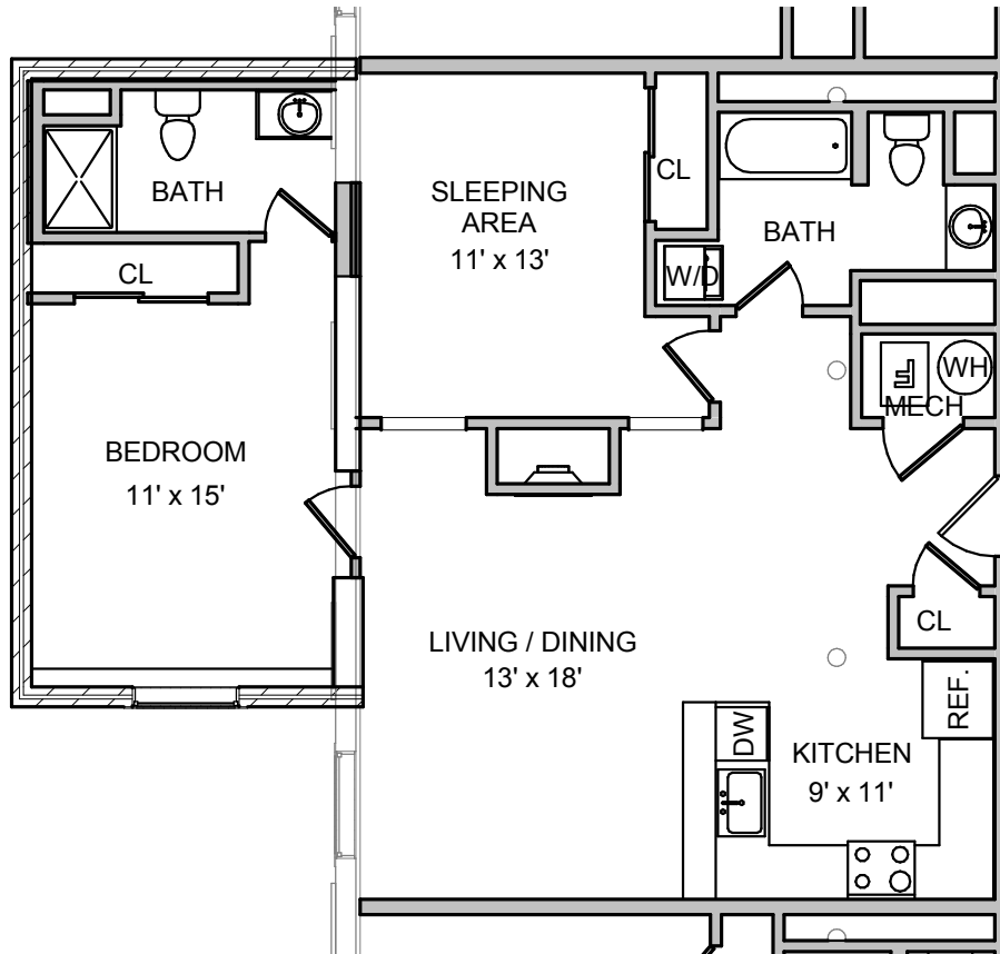
① C306 1/8" = 1'-0" SIMILAR TO UNIT C406
