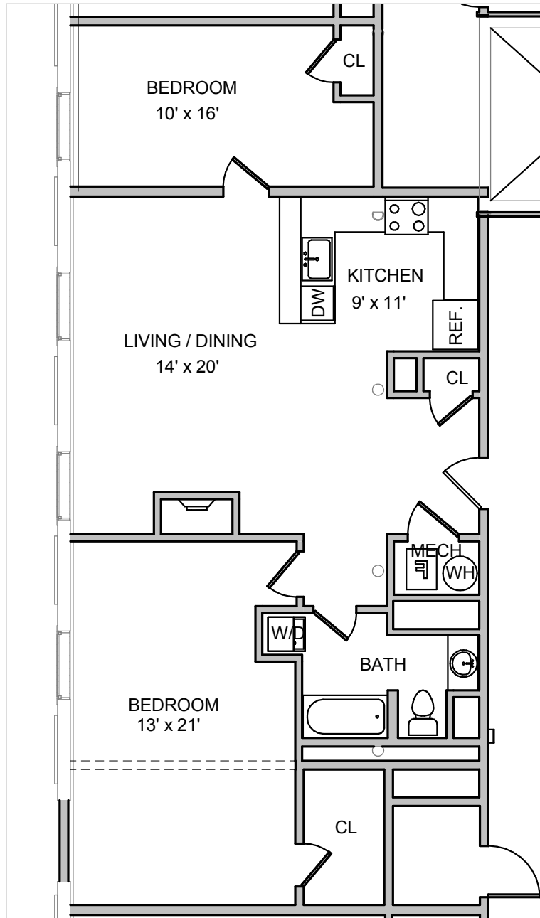
① C302 1/8" = 1'-0" SIMILAR TO UNIT C402
