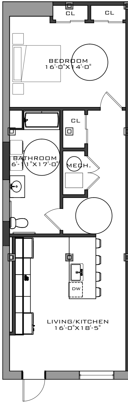
① UNIT TYPE 9 - 808 SF 1/8" = 1'-0"
