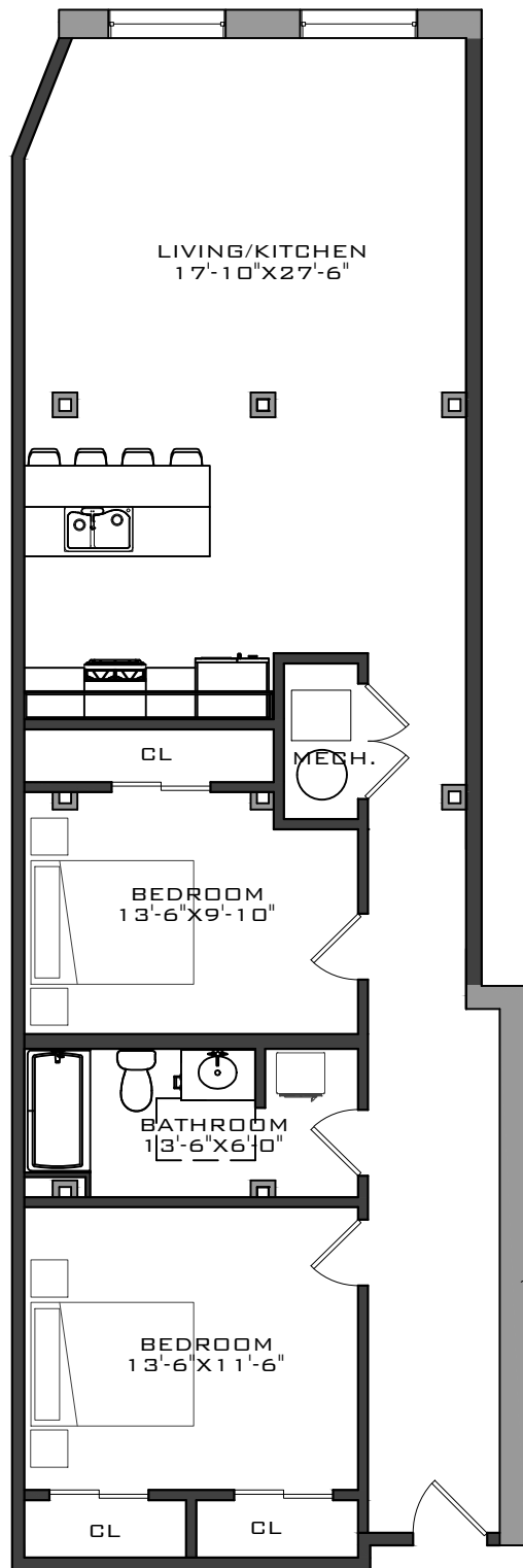
① UNIT TYPE 2 - 1,152 SF 1/8" = 1'-0"
