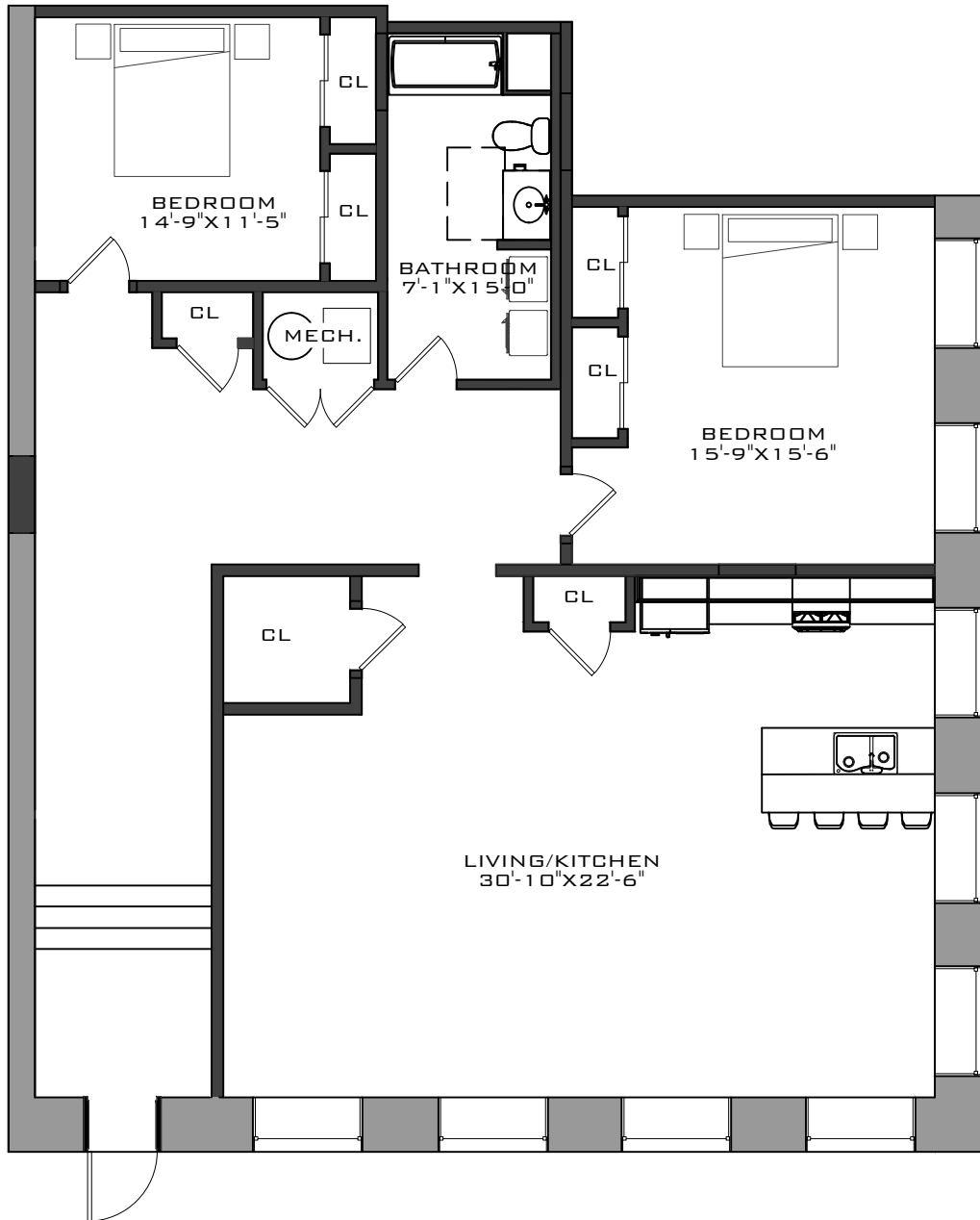
① UNIT TYPE 7 - 1,685 SF 1/8" = 1'-0"
